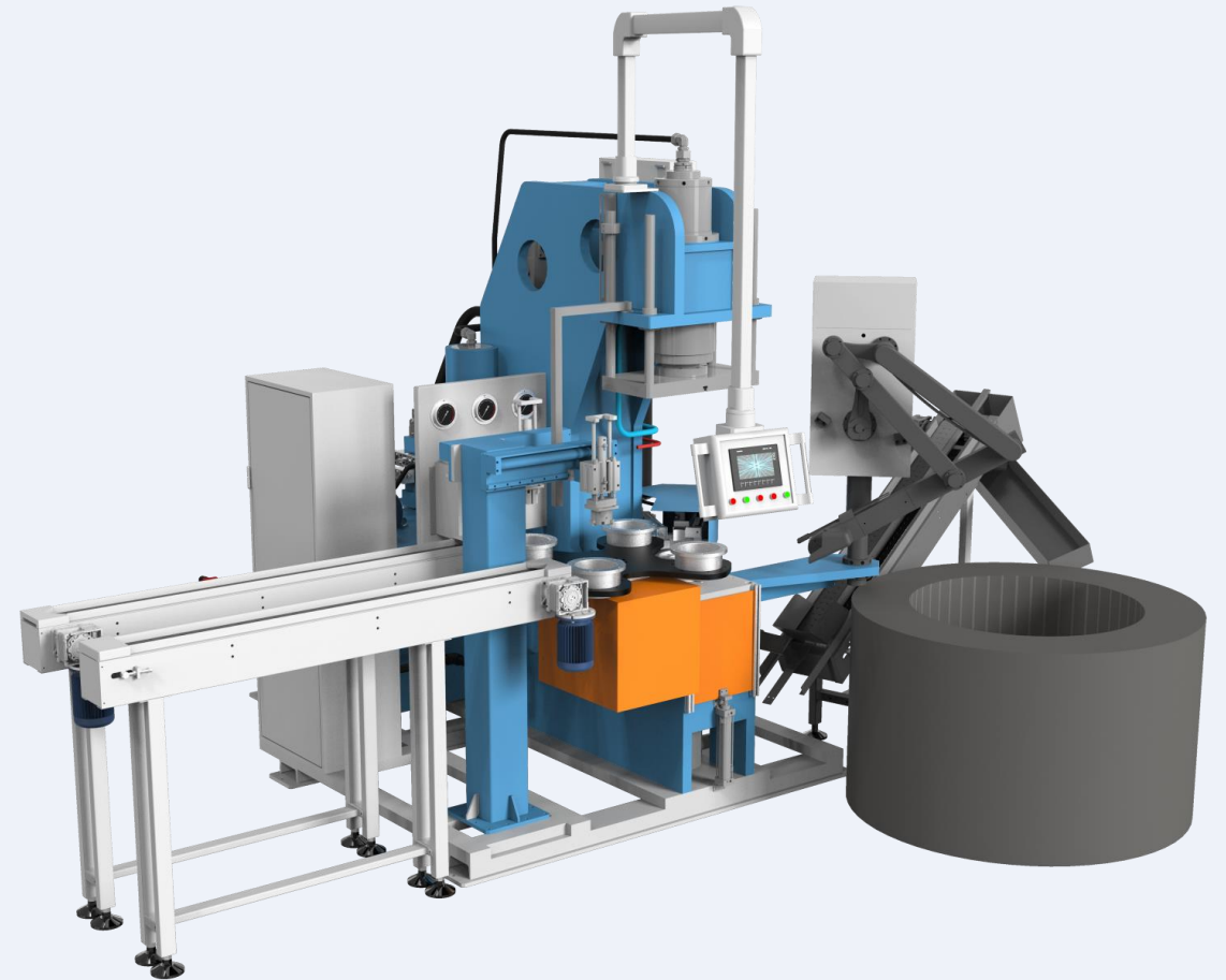
Automatic four-station aluminum rotor casting machine
