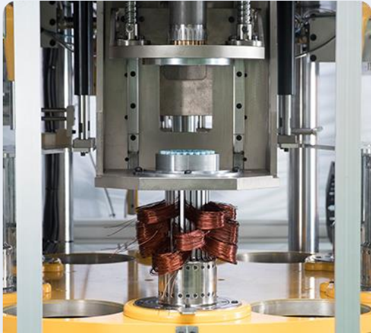
Motor manufacturing machines
