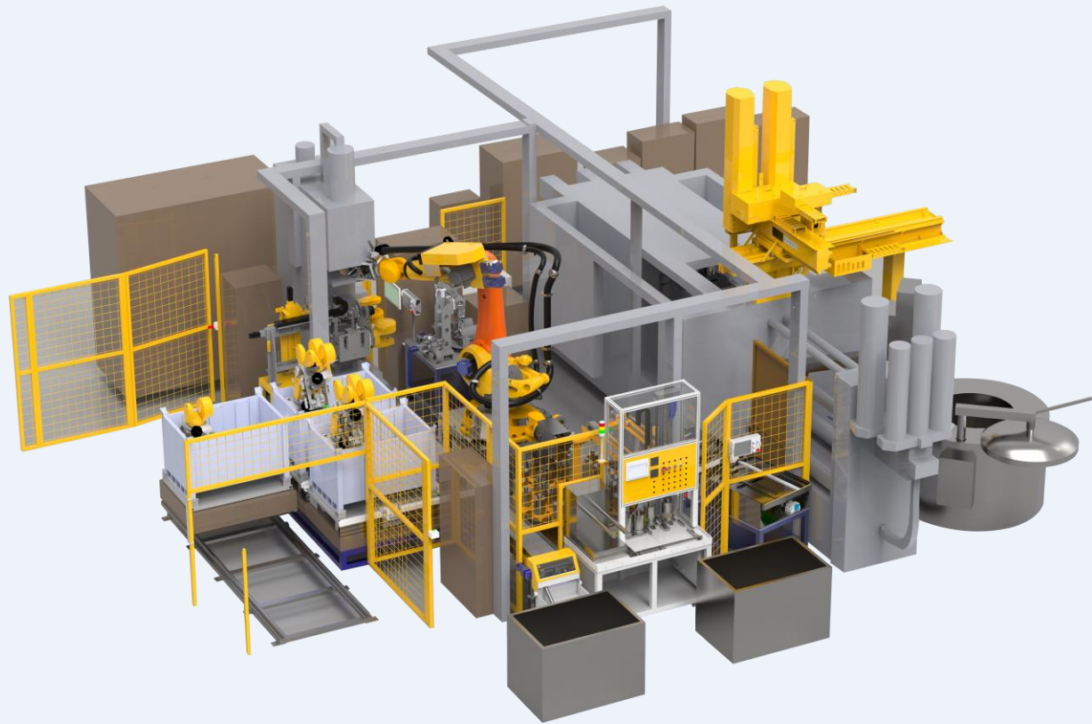
Aluminum rotor casting automatic production line
