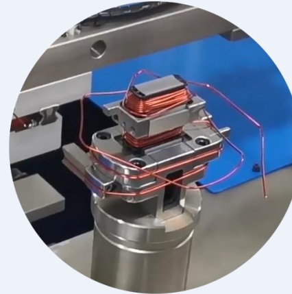
Segment winding
